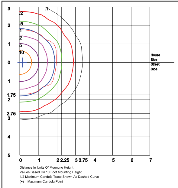
9044AMF1X167UAMC- Type V Grid in MH MH=10 Feet
