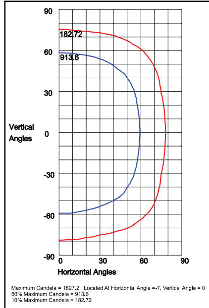
9044AMF1X167UAMC 115H x 110V, NEMA 7H x 7V
